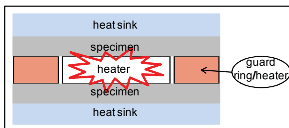
Figure 7.33 Guarded hot-plate set up
