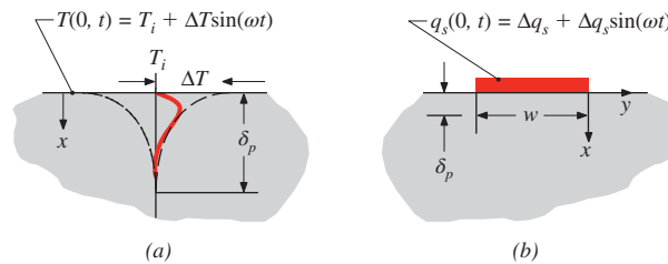
FIGURE 5.11 Schematic of (a) a periodically heated, one-dimensional semi-infinite solid and (b) a periodically heated strip attached to a semi-infinite solid.
