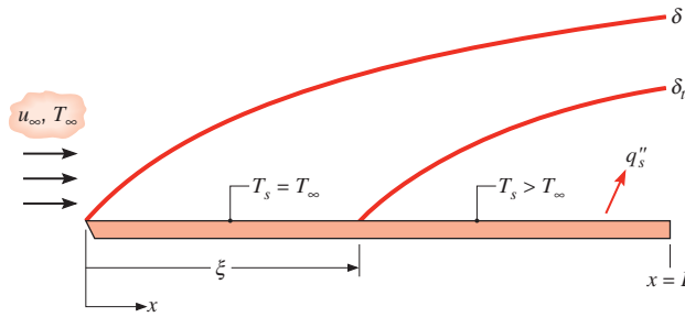
FIGURE 7.5 Flat plate in parallel flow with unheated starting length.
