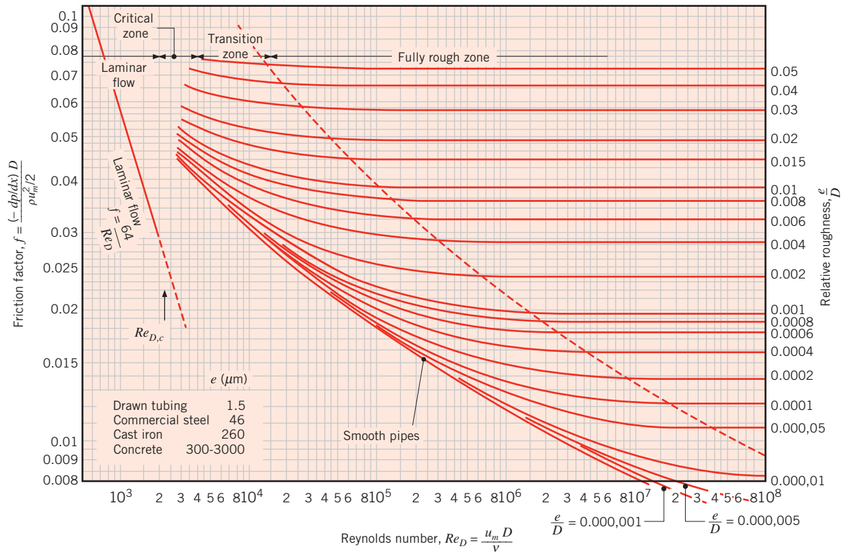
FIGURE 8.3 Friction factor for fully developed flow in a circular tube. Used with permission from Moody, L. F., Trans. ASME , 66 , 671, 1944.
