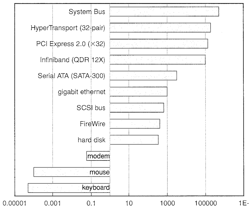
Figure 13.10 Sun Enterprise 6000 device-transfer rates (logarithmic).
