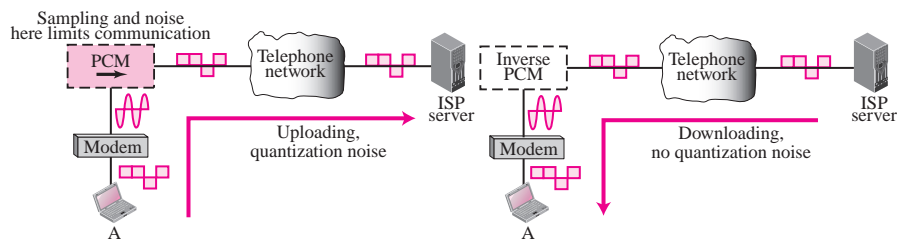
Figure 3.26 56K modem
