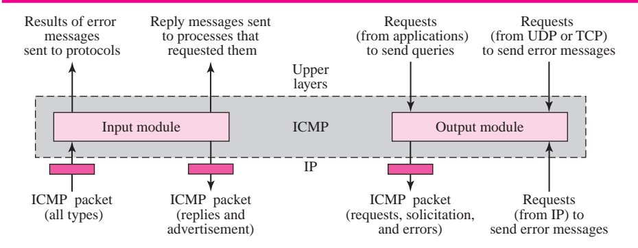
Figure 9.16 ICMP package
