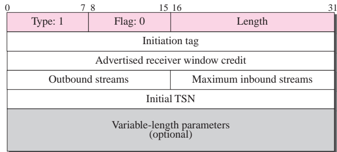
Figure 16.10 INIT chunk
