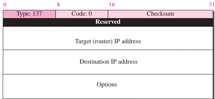
Figure 28.14 Redirection message
