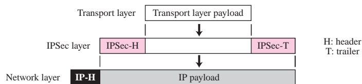
Figure 30.1 IPSec in transport mode
