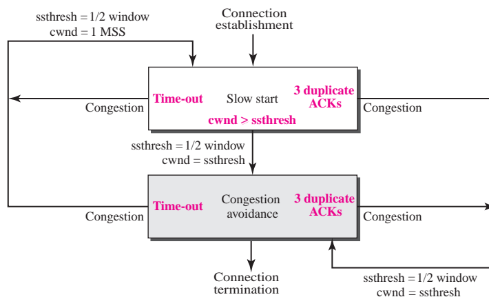
Figure 15.36 TCP congestion policy summary
