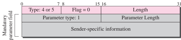
Figure 16.15 HEARTBEAT and HEARTBEAT ACK chunks
