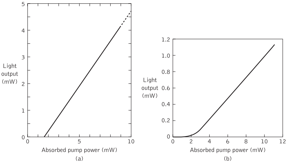
Figure 6.48 Light output against absorbed pump power characteristics for fiber lasers. (a) Neodymium-doped silica fiber. Reproduced with permission from M. Shimizu, H. Suda and M. Horiguchi, 'High efficiency Nd-doped fibre lasers using direct-coated dielectric mirrors', Electron. Lett. , 23 , p. 768, 1987 (IEE). (b) Erbium/ytterbium with alumina codoped silica fiber. Reproduced with permission from D. N. Payne and L. Reekie, 'Rare-earth-doped fibre lasers and amplifiers', IEE Conf. Publ. , 292 , Pt 1, p. 49, 1988
