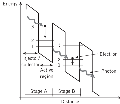
Figure 6.60 Energy-level diagram for a quantum cascade laser
