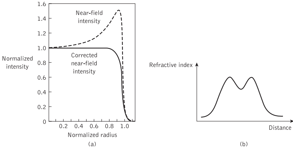
Figure 14.18 (a) The refractive index profile of a step index fiber measured using the near-field scanning method, showing the near-field intensity and the corrected near-field intensity. Reproduced with permission from F. E. M. Sladen, D. N. Payne and M. J. Adams, Appl. Phys. Lett. , 28 , p. 225, 1976 © 1976, American Institute of Physics. (b) The refractive index profile of a practical step index fiber measured by the near-field scanning method [Ref. 47]
