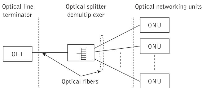
Figure 15.38 General structure of a passive optical network (PON)
