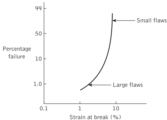
Figure 4.20 A schematic representation of a Weibull plot. Reproduced with permission from M. H. Reeve, Radio Electron. Eng. , 51 , p. 327, 1981
