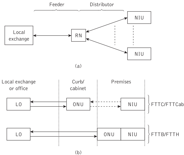
Figure 15.37 Optical fiber access network: (a) feeder and distribution sections; (b) different deployment strategies
