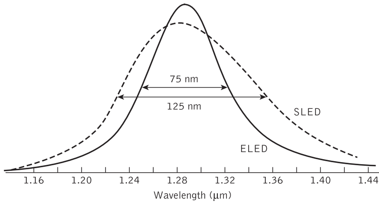
Figure 7.23 Typical spectral output characteristics for InGaAsP surface- and edge-emitting LEDs operating in the 1.3 \mu\text{m} wavelength region [Ref. 13; © Elsevier]
