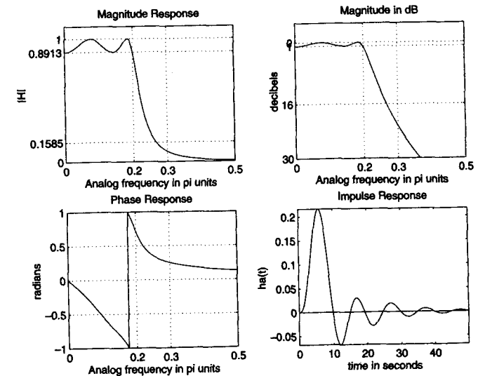
FIGURE 8.6 Chebyshev-I analog filter in Example 8.6
