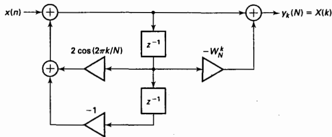
FIGURE 10.15 Realization of two-pole resonator for computing the DFT
