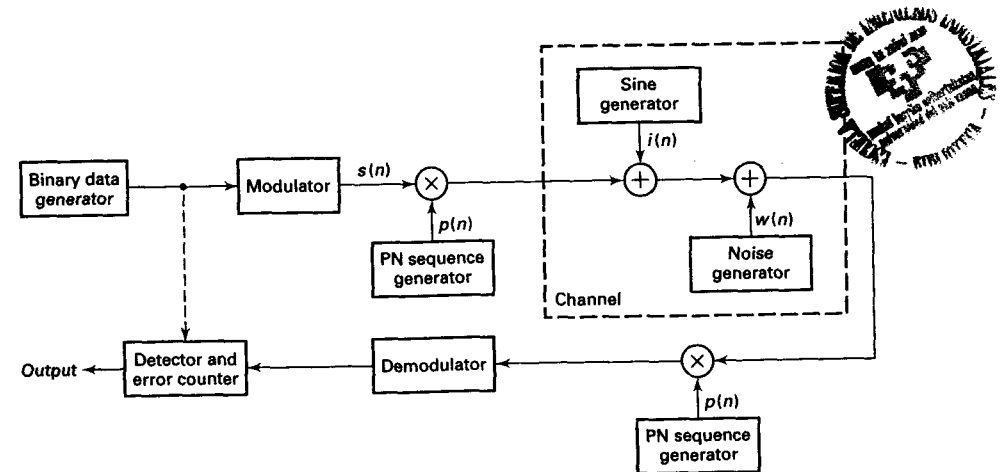
FIGURE 10.18 Block diagram of binary PN spread-spectrum system for simulation experiment
