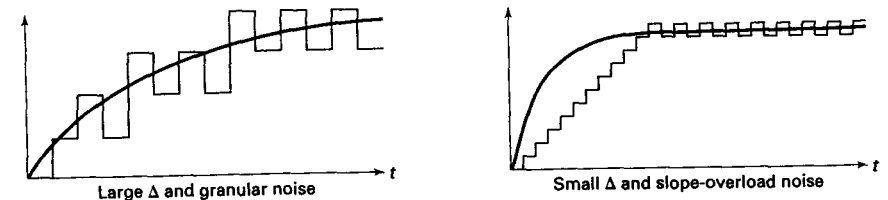
FIGURE 10.10 Two types of distortion in the DM encoder
