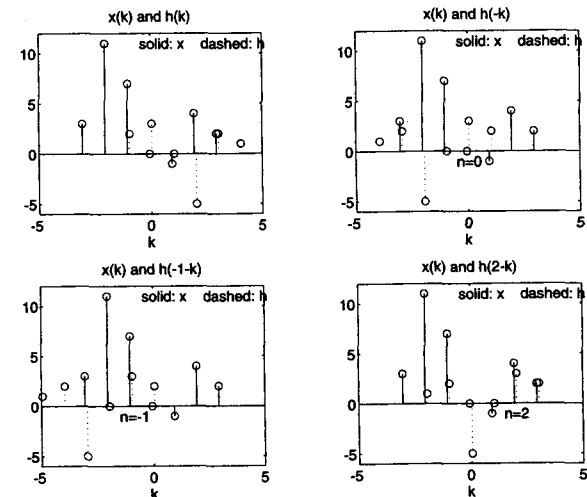
FIGURE 2.7 Graphical convolution in Example 2.6
