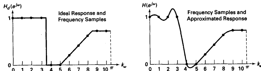
FIGURE 7.25 Pictorial description of frequency sampling technique
