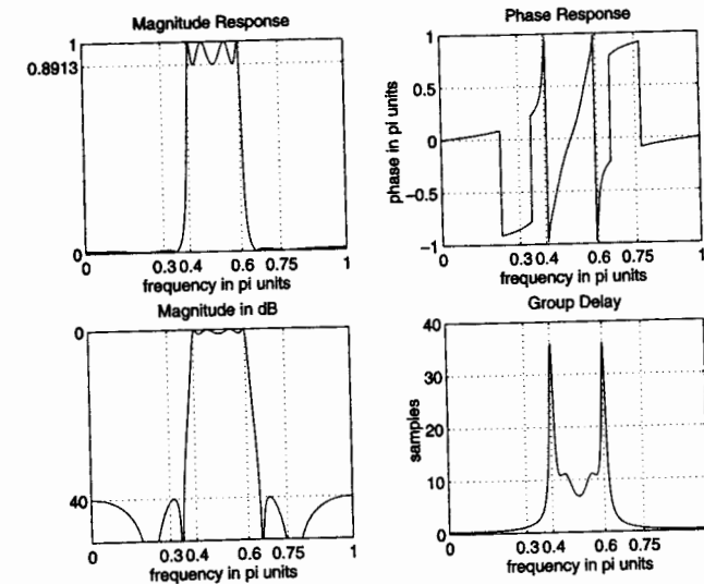
FIGURE 8.23 Digital elliptic bandpass filter in Example 8.29
