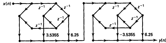
FIGURE 6.14 Cascade of FIR linear-phase elements
