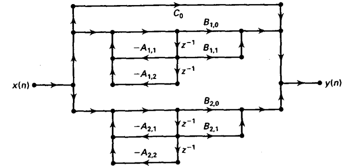
FIGURE 6.7 Parallel form structure for N = 4
