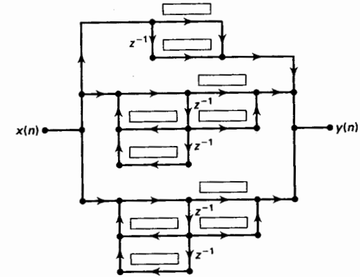
FIGURE 6.26 Structure for Problem 6.6
