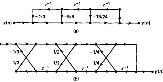
FIGURE 6.21 IIR filter structures in Example 6.9: (a) Direct form (b) Lattice form
