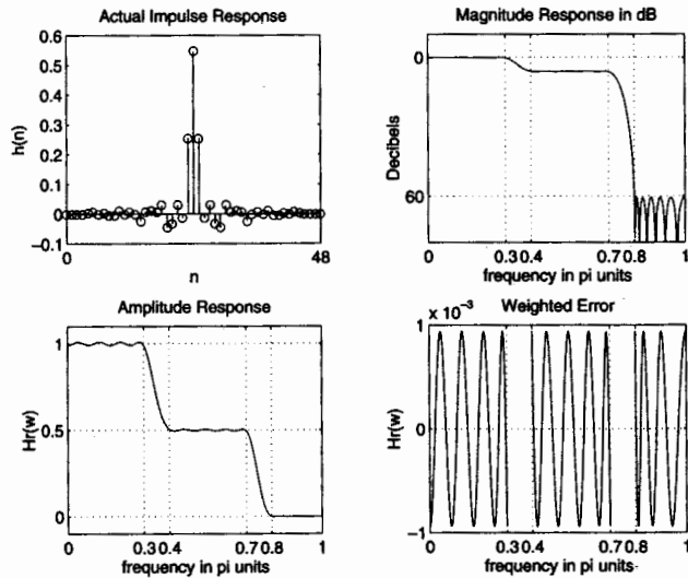
FIGURE 7.38 Plots for equiripple staircase FIR filter in Example 7.26
