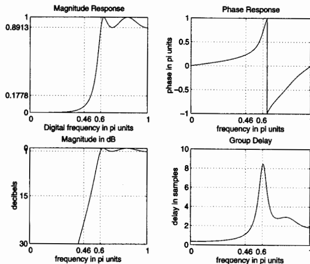
FIGURE 8.22 Digital Chebyshev-I highpass filter in Example 8.28
