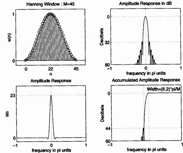
FIGURE 7.12 Hanning window: M = 45
