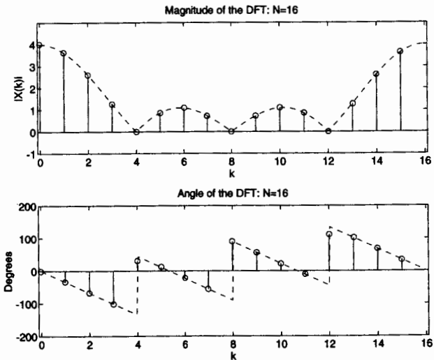
FIGURE 5.7 The DFT plots of Example 5.7: N = 16
