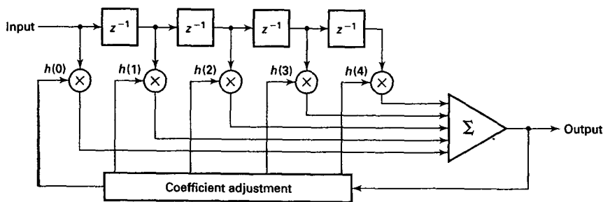
FIGURE 9.1 Direct form adaptive FIR filter
