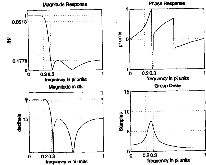
FIGURE 8.18 Digital Chebyshev-II lowpass filter using bilinear transformation
