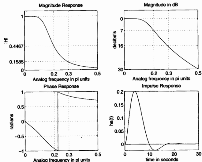
FIGURE 8.5 Butterworth analog filter in Example 8.4
