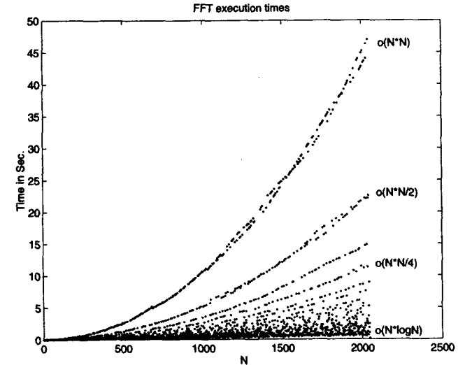
FIGURE 5.20 FFT execution times for 1 \leq N \leq 2048
