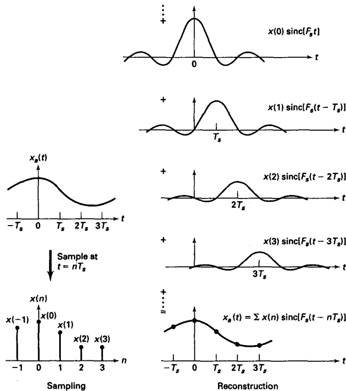
FIGURE 3.14 Reconstruction of band-limited signal from its samples
