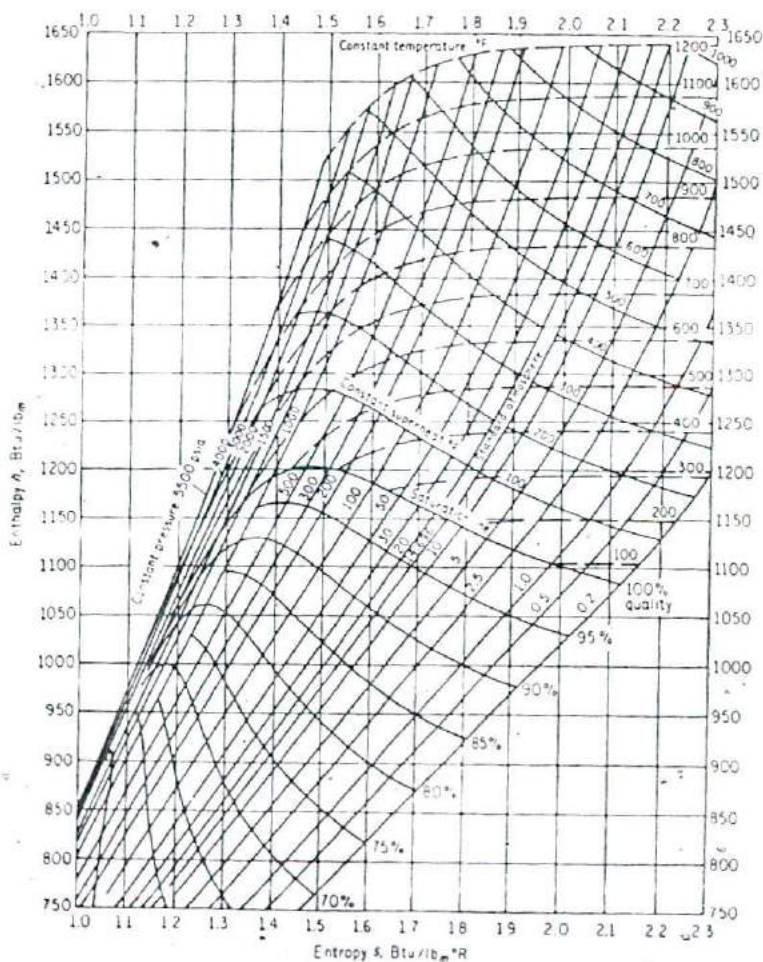
Figure A-1 Mollier diagram for steam. (Based on data in Ref. 6.)
